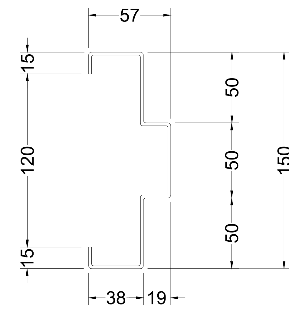
FRAME PROFILE
