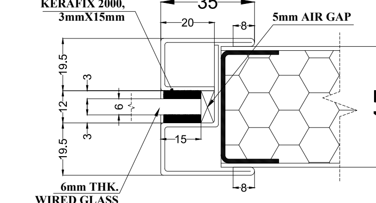
DETAIL OF VISION GLASS BOTTOM EDGES
