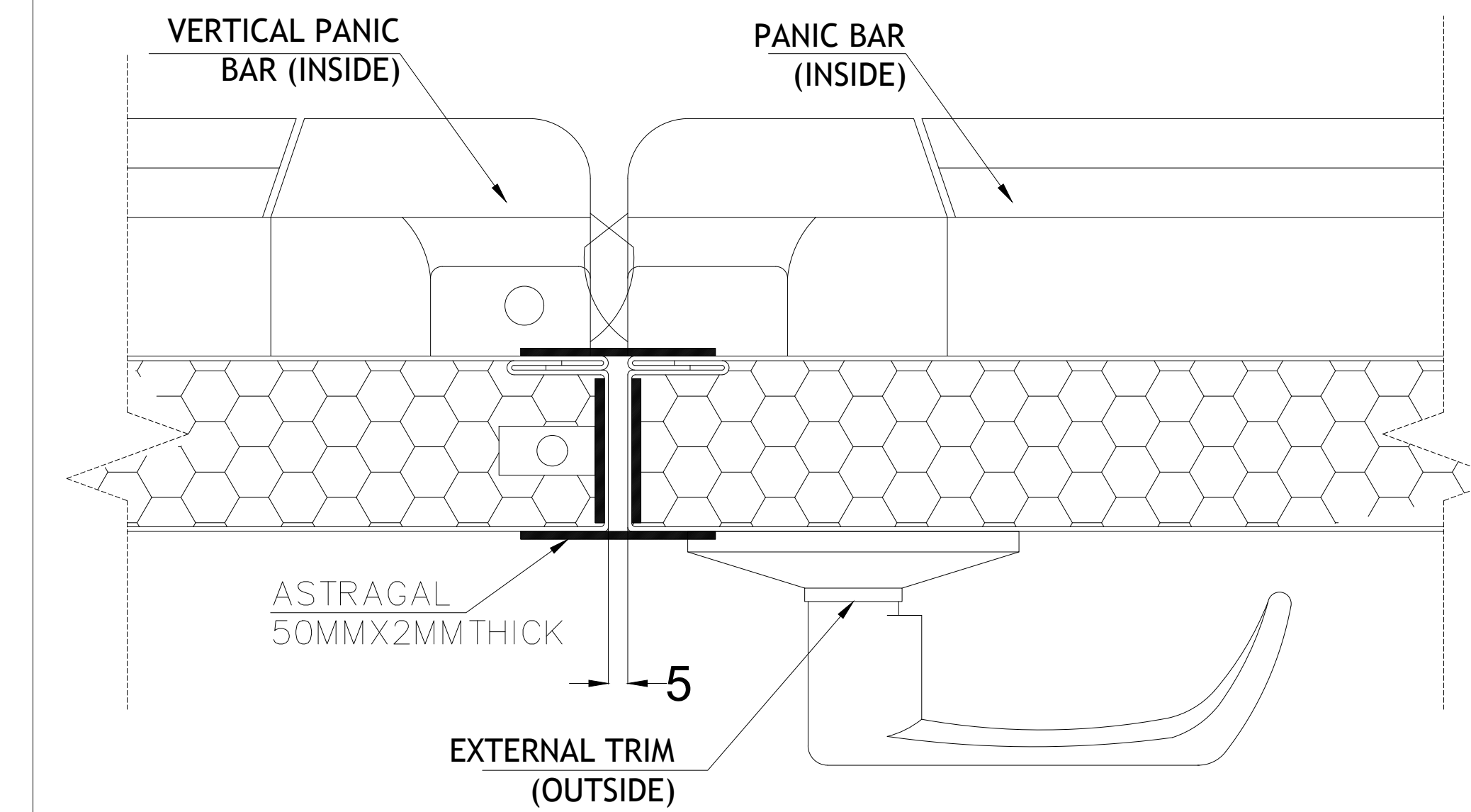
ASTRAGAL DETAILS (DETAIL "D")
