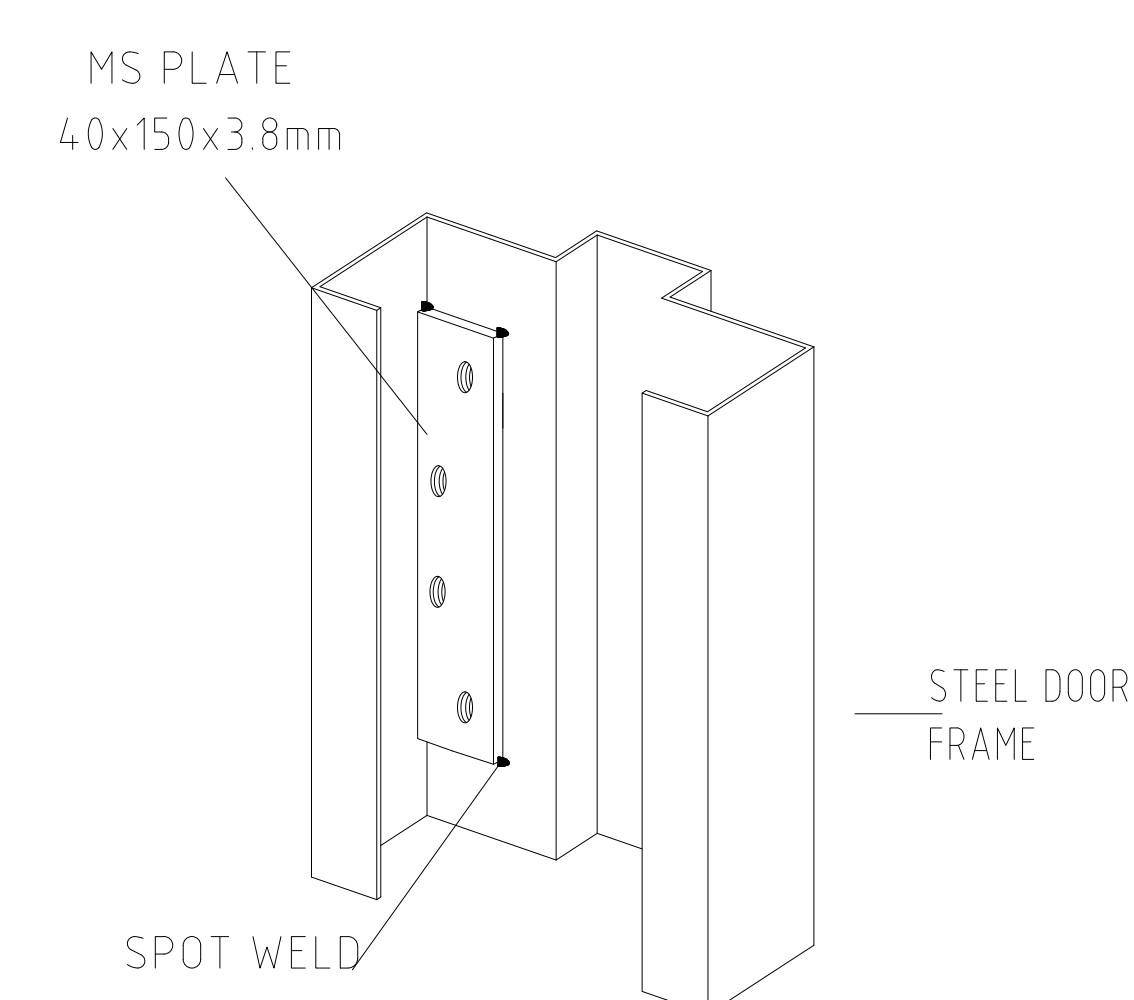
HINGE REINFORCEMENT DETAIL
