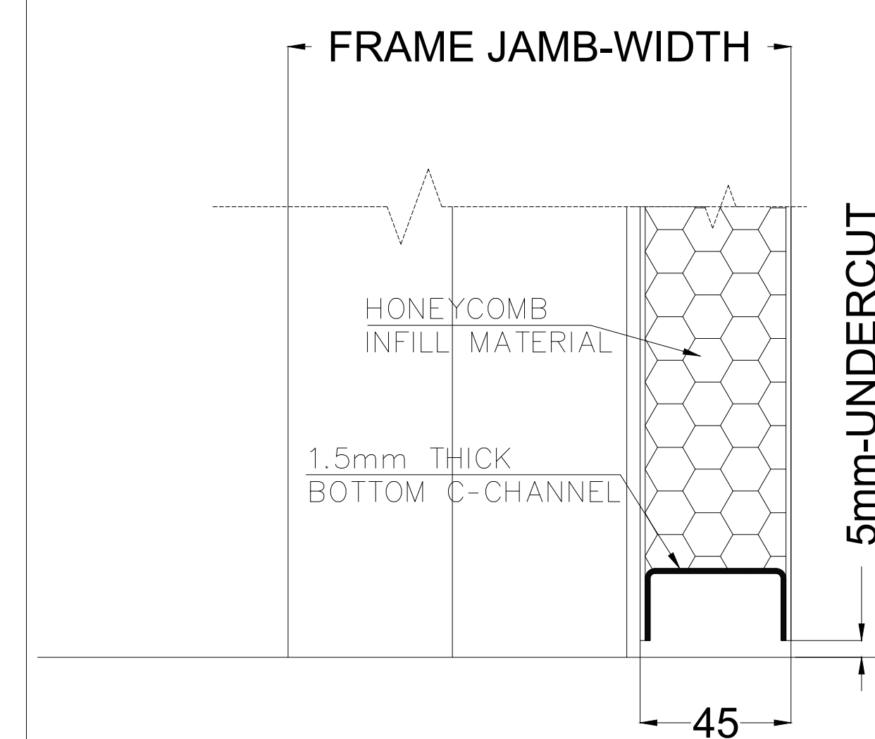
BOTTOM CHANNEL DETAILS (DETAIL "C")
