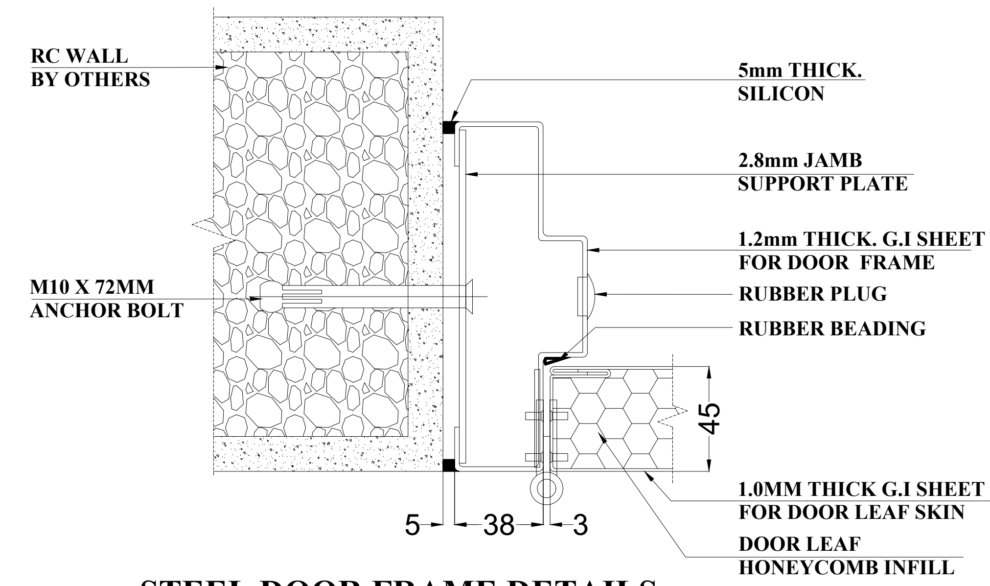
STEEL DOOR FRAME DETAILS (DETAIL "A"
