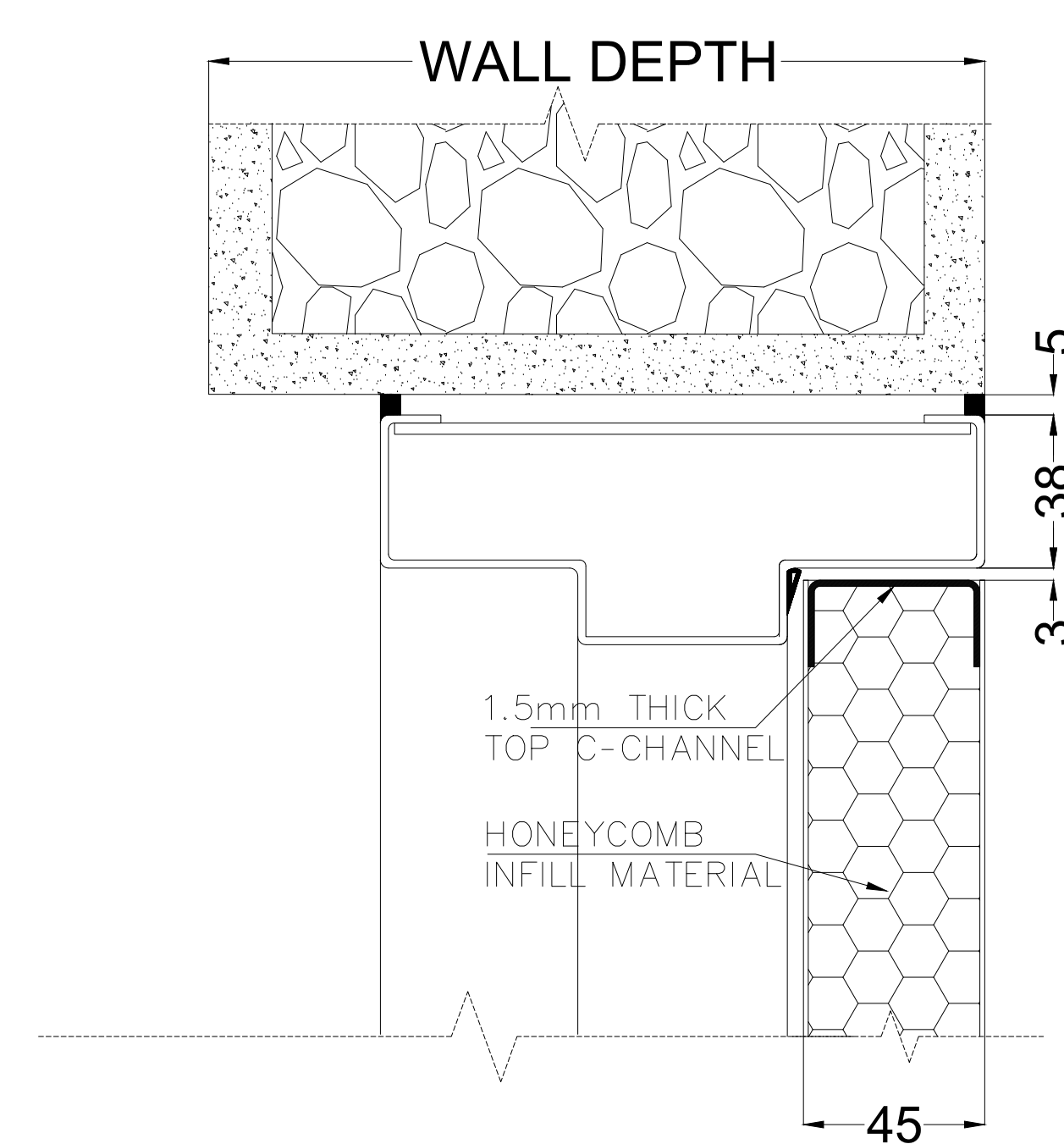
TOP CHANNEL DETAILS (DETAIL "B")
